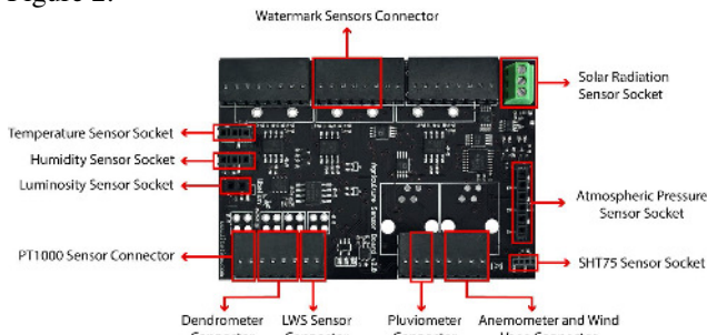
Figure 2: Upper side of Waspnote agriculture board
