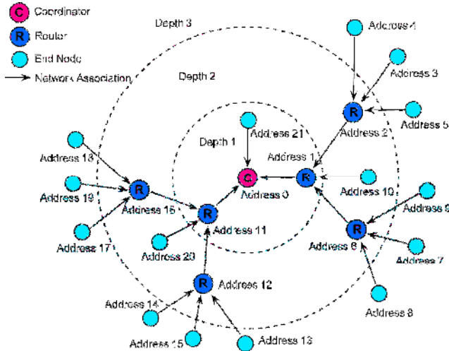
Figure 3: Cluster tree topology
