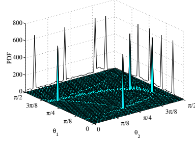
Fig. 2. Histogram of angles for the measurements of Figure 1. The (m - 1) -dimensional projections onto the plane of angle \theta_i , i = 1, \dots, m - 1 are also shown.
