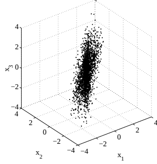
Fig. 1. Scatter plot of measurements for a scenario with three sensors ( m = 3 ) and four sources ( n = 4 ) of sparsity factor: 0.5.
