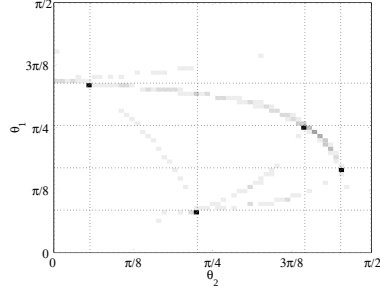
Fig. 3. Top view of the (m - 1) -dimensional PDF corresponding to the spherical angles of the measurements. The black spots correspond to the locations of the maxima from Figure 2.
