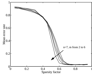
Fig. 5. Mean error rate for scenarios with a fixed number of seven sources and a number of sensors ranging from two to six, as a function of the sparsity factor of the sources.
