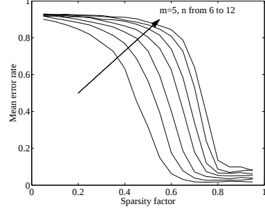
Fig. 4. Mean error rate for scenarios with a fixed number of five sensors and a number of sources ranging from six to twelve, as a function of the sparsity factor of the sources.
